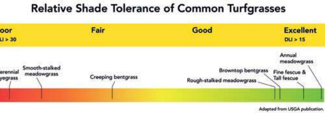
Figure 1 - Relative Shade Tolerance of Common Turfgrasses
